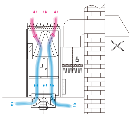
Mechanical Cooling Mode
