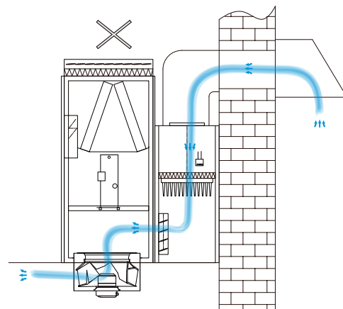
Free Cooling Mode
